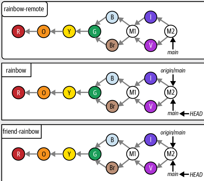
The Rainbow project at the start of Chapter 11 with all the commits since Chapter 1
