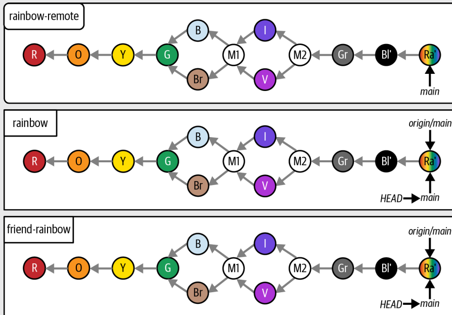
The Rainbow project at the end of Chapter 11 with all the commits since Chapter 1
