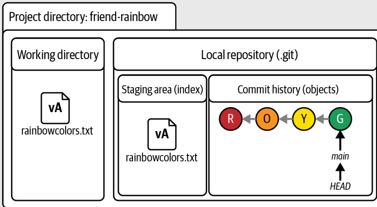
Git Diagram showing the current state of the friend-rainbow project directory
