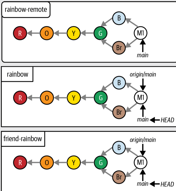
The Rainbow project at the start of Chapter 10 with all the commits since Chapter 1
