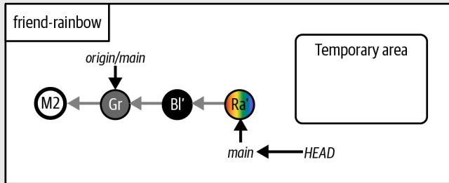
Stage 5: Switch onto the branch you rebased
