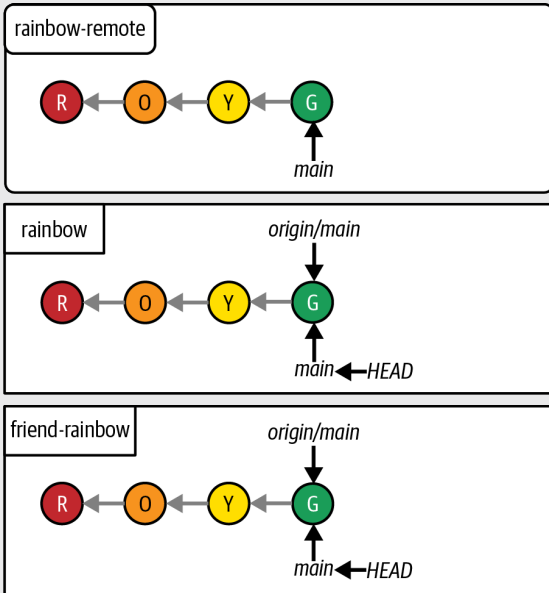
The Rainbow project at the start of Chapter 9 with all the commits since Chapter 1
