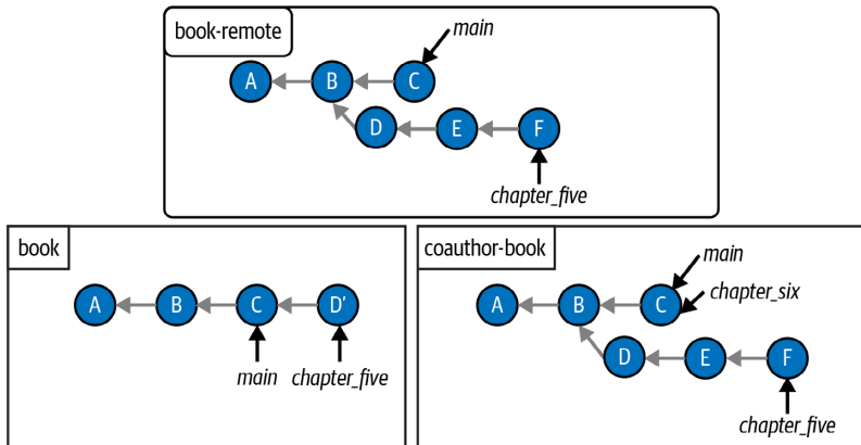
FIGURE 11-11 The Book project after my coauthor contributes to the remote chapter_five branch
