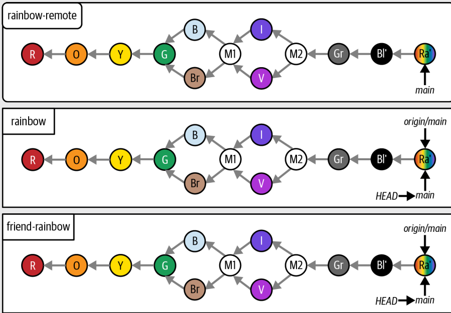
The Rainbow project at the start of Chapter 12 with all the commits since Chapter 1
