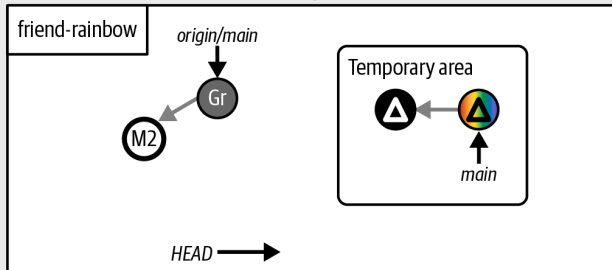
Stage 2: Save information about the rebase in a temporary area
