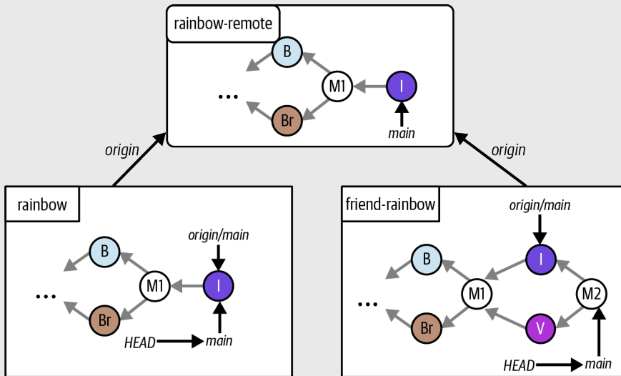
The Rainbow project after your friend resolves the merge conflicts in the friend-rainbow repository and makes another merge commit
