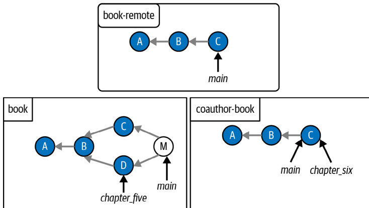
FIGURE 11-3 The Book project if I were to integrate the changes from the remote repository using a three-way merge
