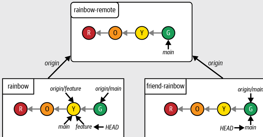
The Rainbow project after you fetch the data from the rainbow-remote repository to the rainbow repository
