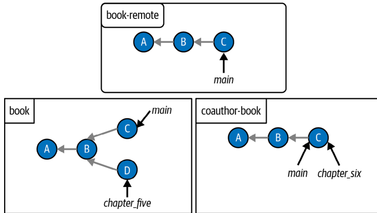
FIGURE 11-4 The Book project after I pull the changes from the remote main branch
