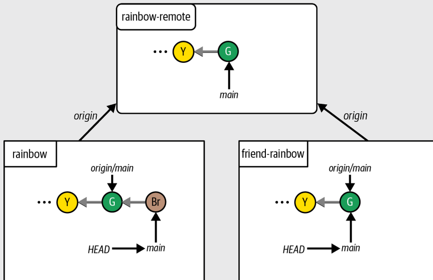
The Rainbow project after you make the brown commit in the rainbow repository
