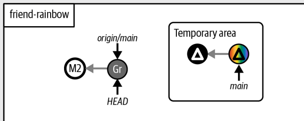
Stage 3: Reset HEAD to the same commit as the branch you are rebasing onto (here, the gray commit)
