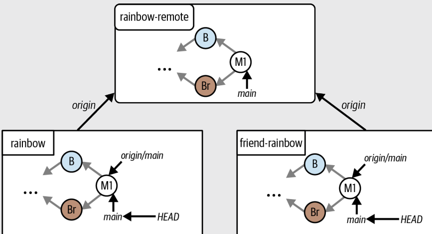
A simplified representation of the Rainbow project at the start of Chapter 10, showing just the last three commits on the main branch in all the repositories
