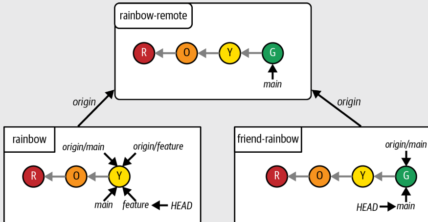
The Rainbow project after your friend pushes the green commit to the remote repository
