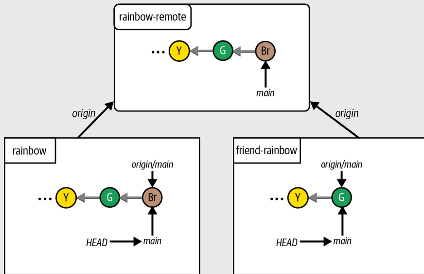
The Rainbow project after you push your local main branch to the rainbow-remote repository
