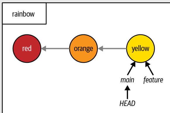
The rainbow repository at the start of Chapter 7
