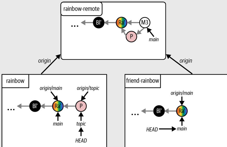
The Rainbow project after you delete the remote topic branch
