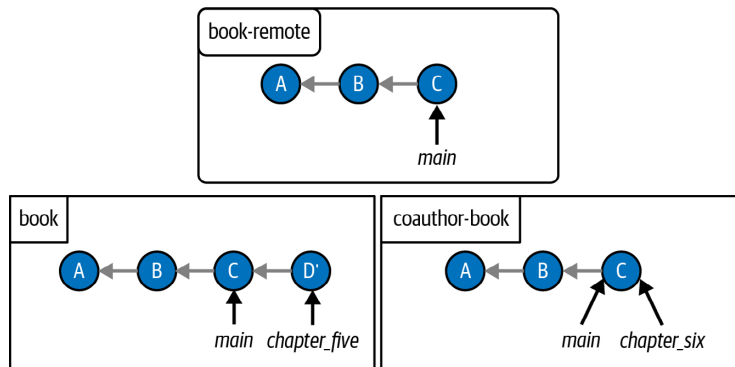
FIGURE 11-5 The Book project after I integrate the changes from the remote repository by rebasing my chapter_five branch onto the main branch
