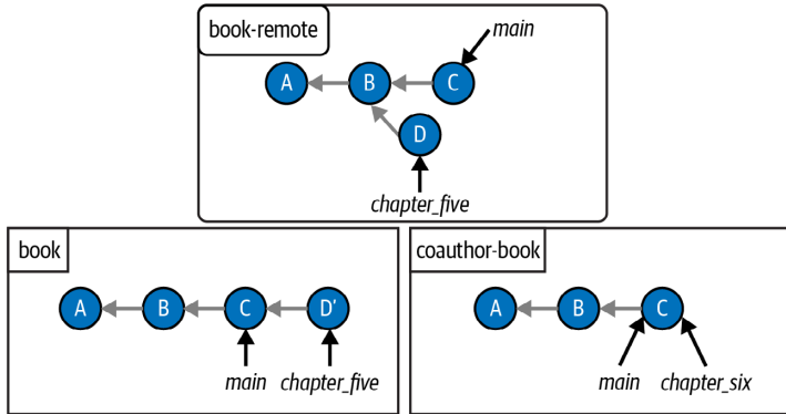
FIGURE 11-10 The Book project after I rebase the chapter_five branch onto the main branch
