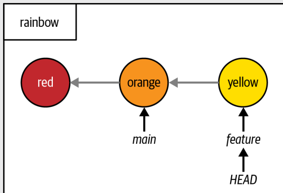
Parent links in the rainbow repository
