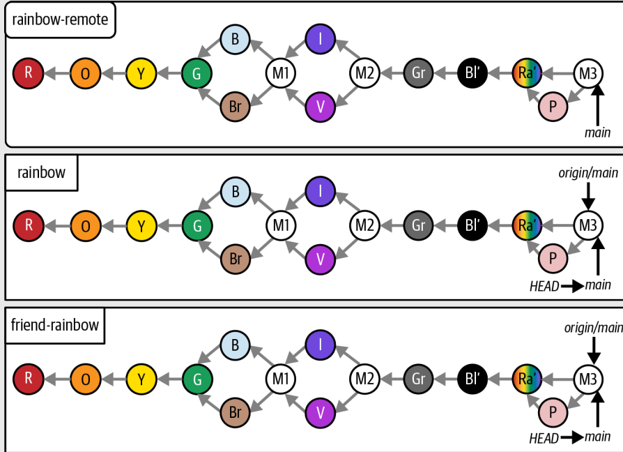
The Rainbow project at the end of Chapter 12 with all the commits since Chapter 1
