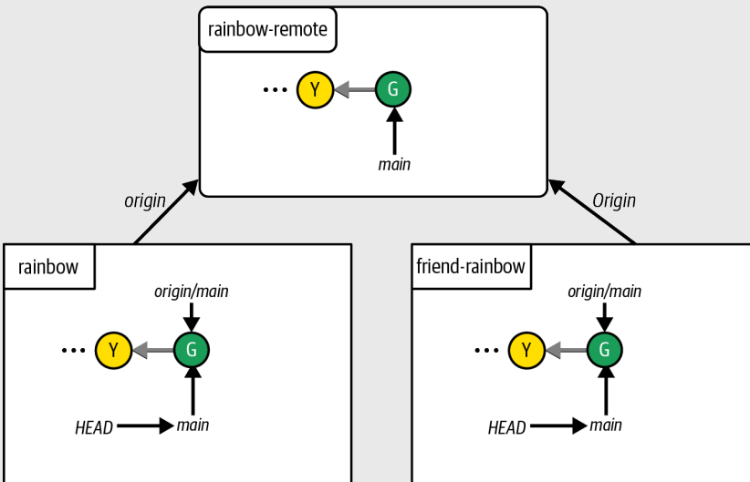
A simplified representation of the Rainbow project at the start of Chapter 9, showing just the last two commits on the main branch in all the repositories
