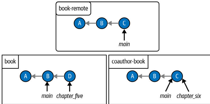
FIGURE 11-2 The Book project after my coauthor pushes their changes to the remote repository
